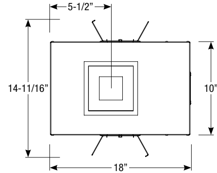
Ceiling Cut-out: 5-3/8" x 5-3/8"
