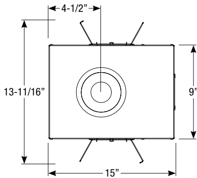
Ceiling Cut-out: 4-3/8" Ø
